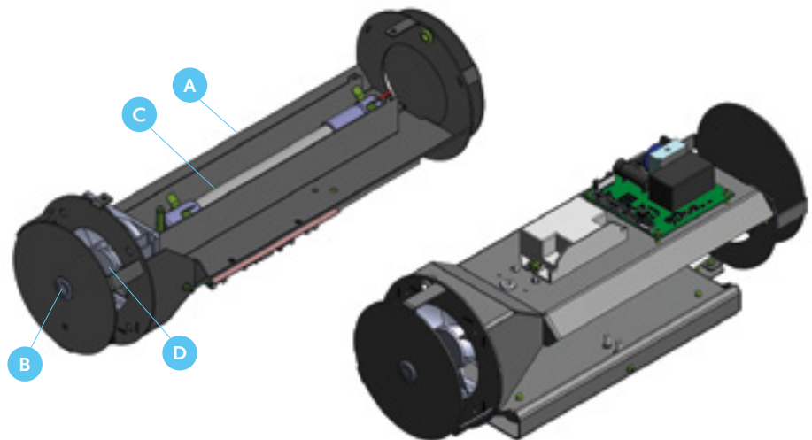
A Case · B On/Off button with blue control light · C UV-C special bulb · D Fan
